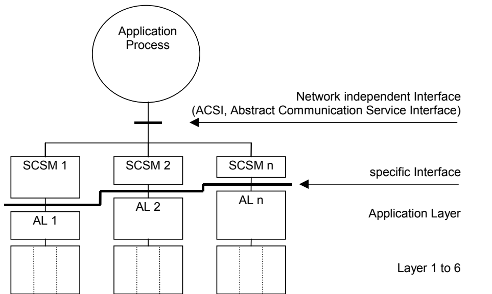
Figure G.3 – ACSI mapping to communication stacks/profiles
