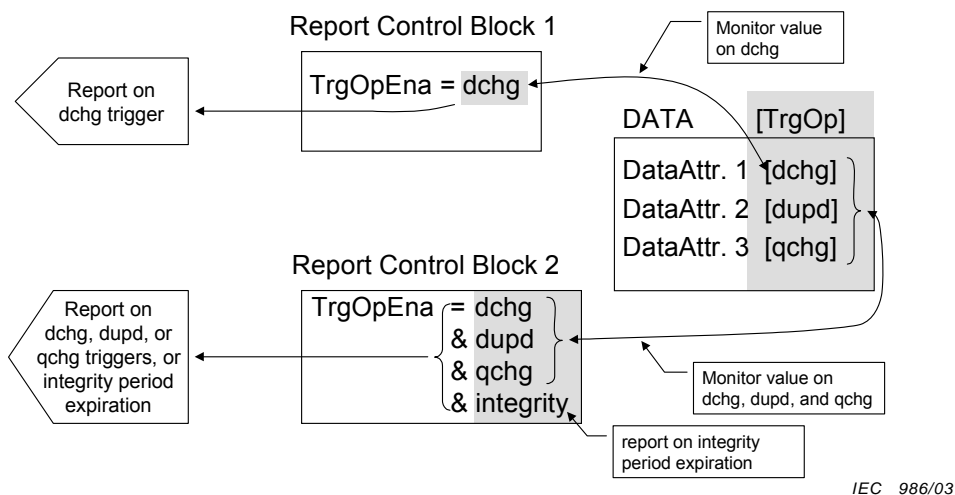
Figure 62 – Relation of TrgOp and Reporting
