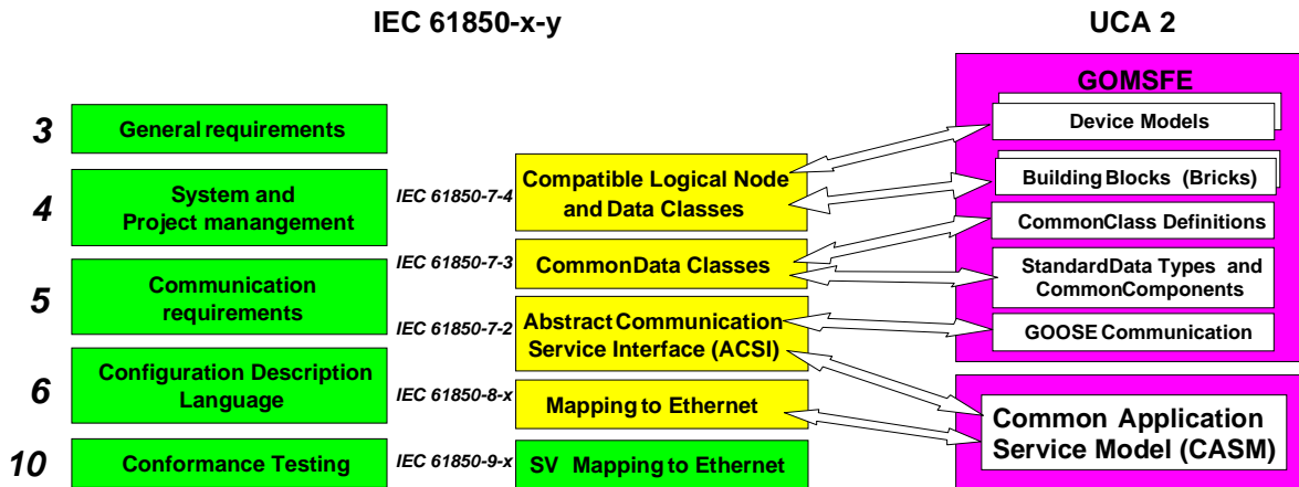
Figure F.1 – Relation between the IEC 61850 series and UCA ®
