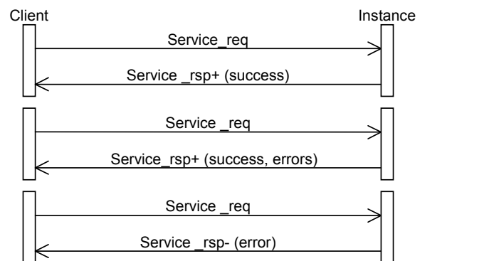
Figure 63 – Sequence diagram
