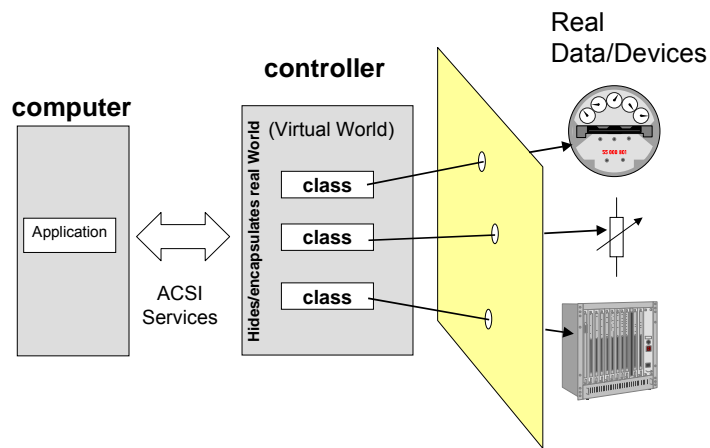
Figure 46 – Virtualisation
