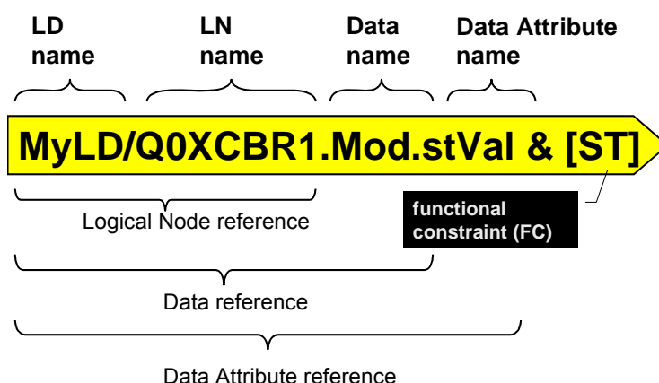
Figure 64 – References
