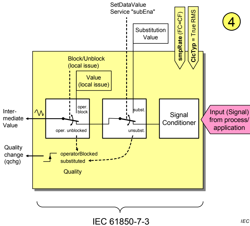
Figure 18 – Input model for analogue values (step 1) (conceptual)
