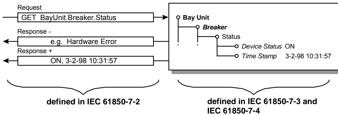
Figure 52 – Example for a service
