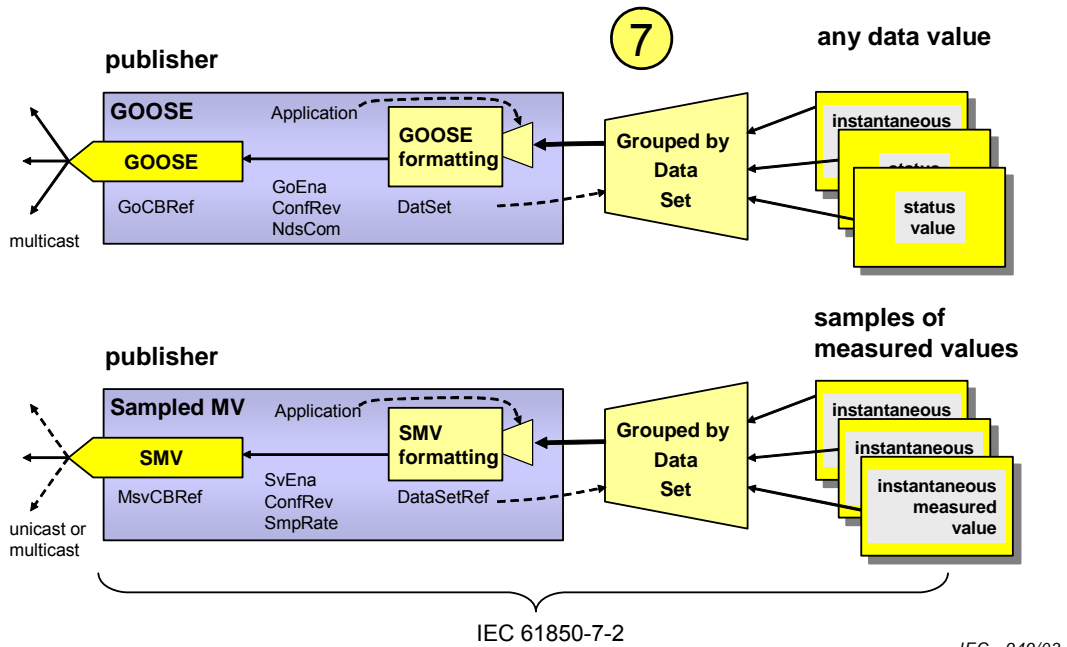
Figure 27 – Peer-to-peer data value publishing model (conceptual)
