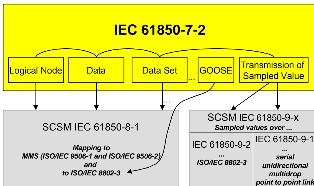
Figure G.2 – ACSI mappings (conceptual)
