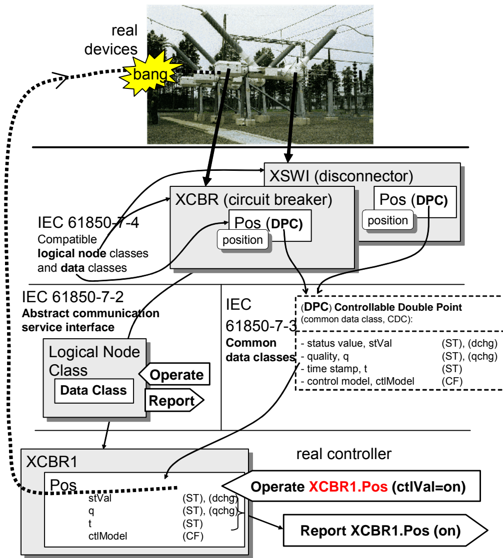
Figure 60 – Relation between parts of the IEC 61850 series
