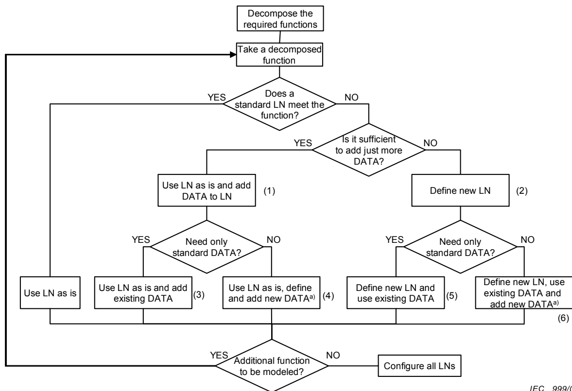
Figure 76 – Basic extension rules diagram
