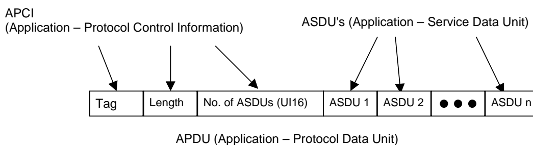
Figure 3 – Concatenation of several ASDU's into one frame
